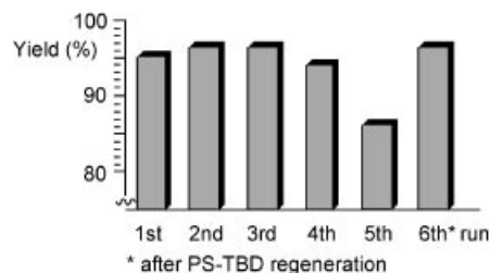
Figure 1. PS-TBD-catalyzed reactions of 1a and 2A . Isolated yield of the mixture of 3aA and 4aA in the re-use of the catalyst.
